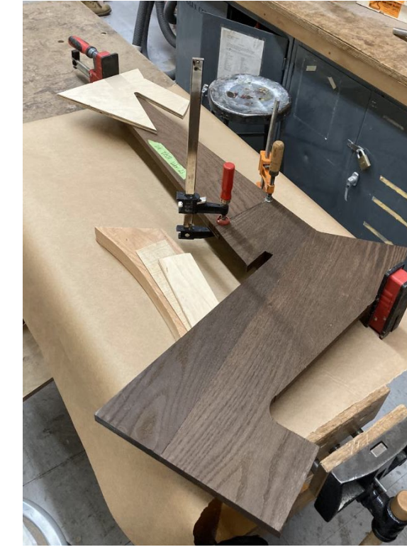
Gluing along lap joint of chair elements
